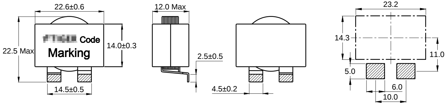
Typical Pad Layout
