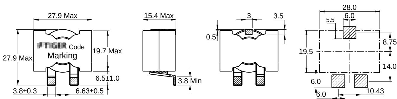
Typical Pad Layout
