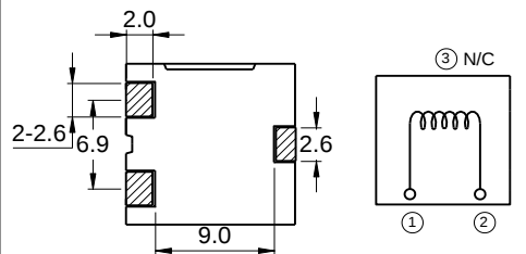
Schematic
