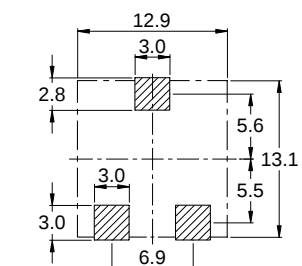
Typical Land Pattern
